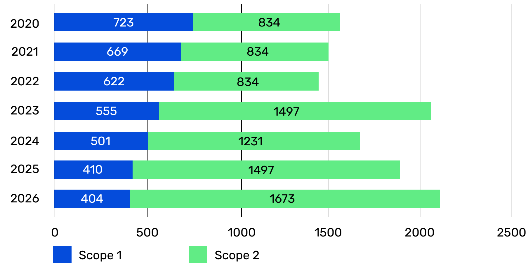
SERO EMS Group CO2e footprint [t]
