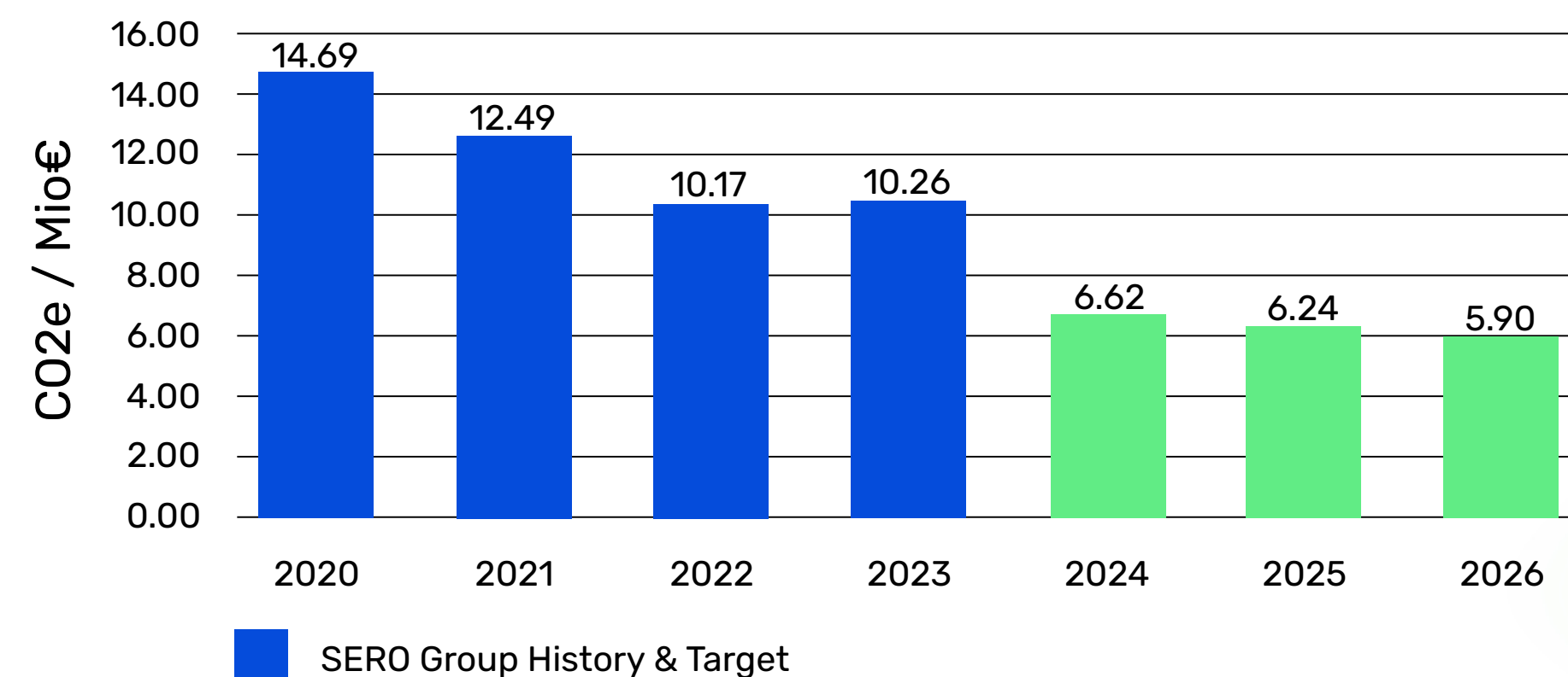
SERO EMS Group - CO2e/Mio Revenue
